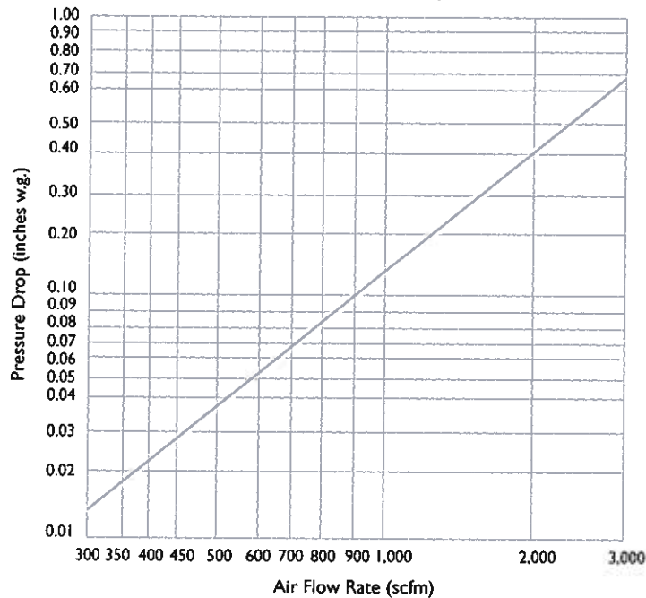
GDC Pressure Drop Data
